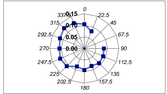
Figure 2. Turbulence intensity at the Fawkner Beacon (17m above MSL)
