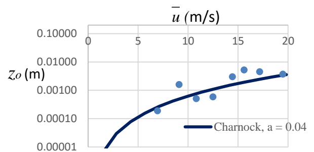
Figure 3. Roughness length versus mean wind speed for northerly winds at Fawkner Beacon
