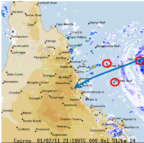
Figure 4. Track of Tropical Cyclone ‘Yasi’ on February 2-3, 2011, showing the automatic weather stations in the Coral Sea ringed in red (map sourced from the Bureau of Meteorology web site).
